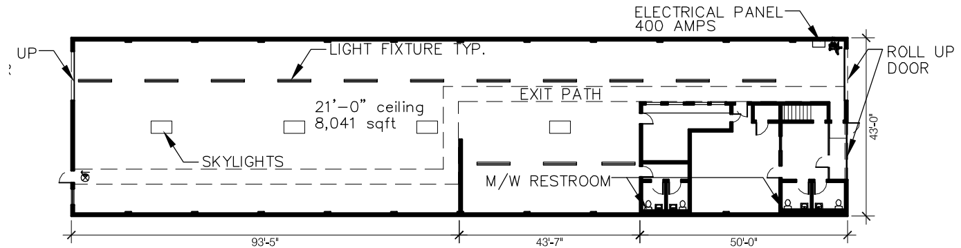
FLOOR PLAN
